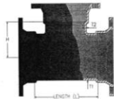
Section A-A D.I. Tee Mechanical Type
